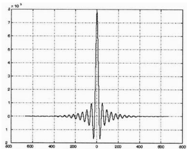
Figure 2. Impulse Response at 96 kHz Sample Rate (X-axis in \mu\text{sec} )
